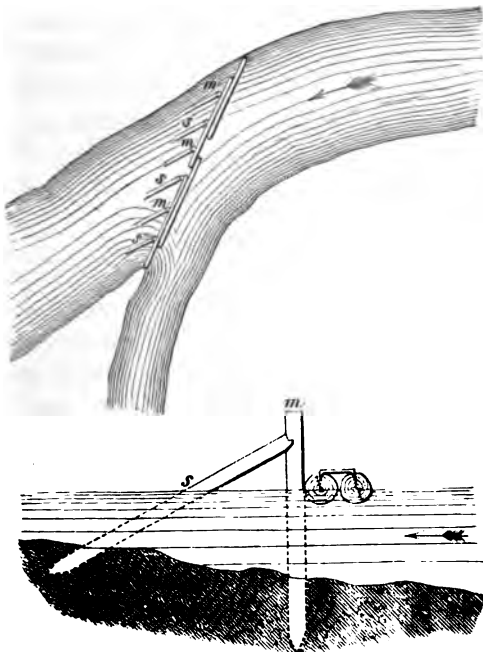
Fig 253.—Fixed lateral boom.
